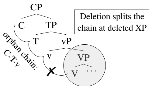
(2) Split-by-deletion
