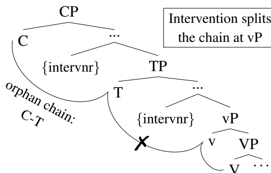
(3) Split-by-intervention
