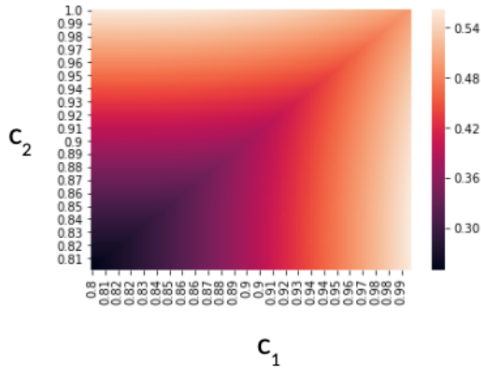
Figure 6: The heatmap shows the marginal probability L_2(w = T|u = No) , as the values of the hyperprior c_1, c_2 are varied. Brighter regions correspond to values of the hyperprior where L_2(w = T|u = No) is higher. These are the values for which No receives an ironic interpretation.
