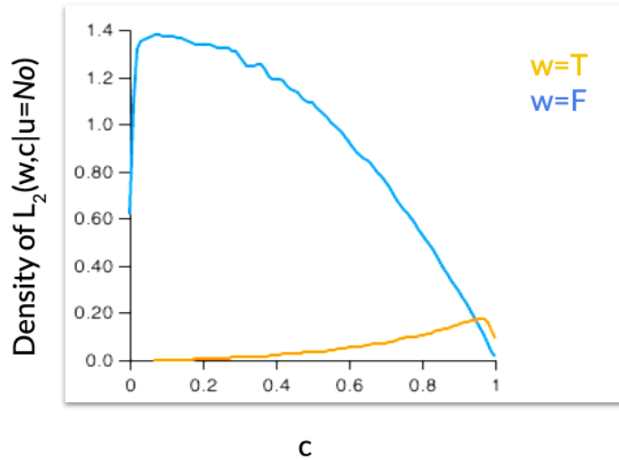
Figure 5: This figure shows the MCMC approximation of L_2(\cdot|u = No) when P_{hyp} is a Beta distribution with \alpha = 1, \beta = 1 . The mode corresponding to pattern 1 is the apex of the left hand curve, with the mode corresponding to pattern 2 is the apex of the right hand curve. Note that the ironic interpretation has low probability, on account of this particular prior assigning insufficiently high marginal probability to T .
