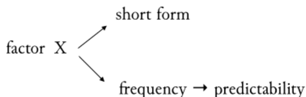
Figure 2: An alternative conception of the causal chain
