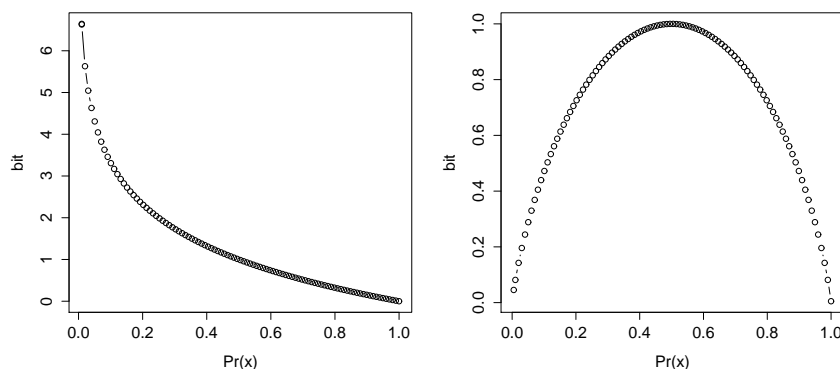
Figure 3: The relationship between the probability of x and its information content (left). The relationship between average entropy (Shannon’s entropy) and the probability of P(x) and P(1-x) (right).
