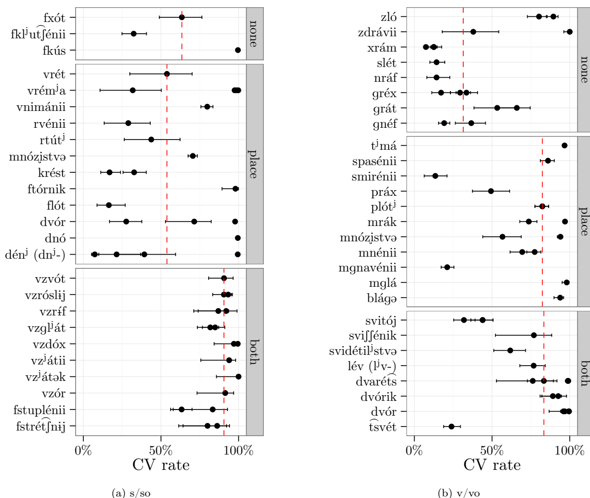
Figure 1: Non-adjacent OCP between the preposition and the word-initial cluster. Error bars indicate 95% binomial confidence intervals. The category “both” includes cases in which one of the consonants in the word-initial cluster has the same manner and place of articulation as the preposition; in “place”, only the place of articulation is shared; and in “none” neither place nor manner are shared. The dashed line represents the median CV rate within each category. Note that for [v/vo] “both” and “place” both have a higher median than “none”, whereas for [s/so] “place” patterns with “none”, and only “both” words show a higher CV rate. 3
